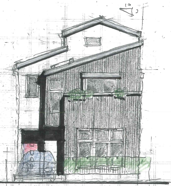
SOUTH ELEVATION
